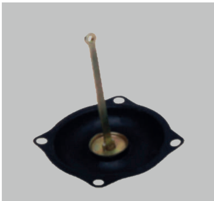
3-01-68 Diafragma Vaccum Toyota 2F
